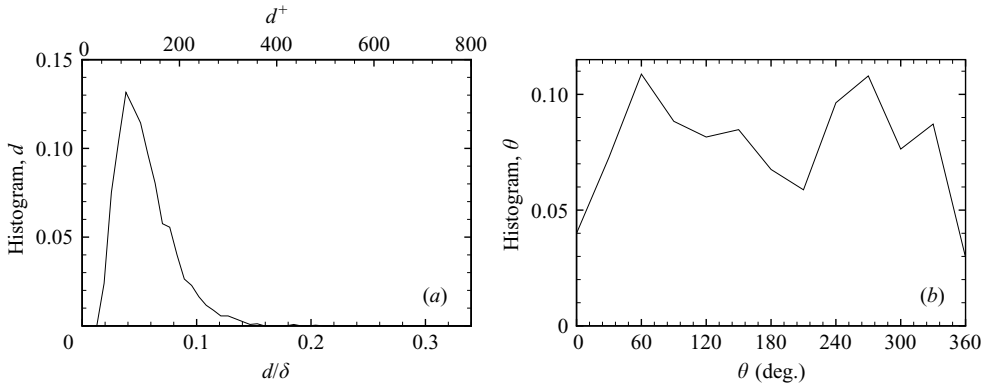
FIGURE 3. Histograms of (a) spacing, d , and (b) angular orientation, \theta , between identified retrograde spanwise vortices at y = 0.2\delta and their closest prograde neighbours.
