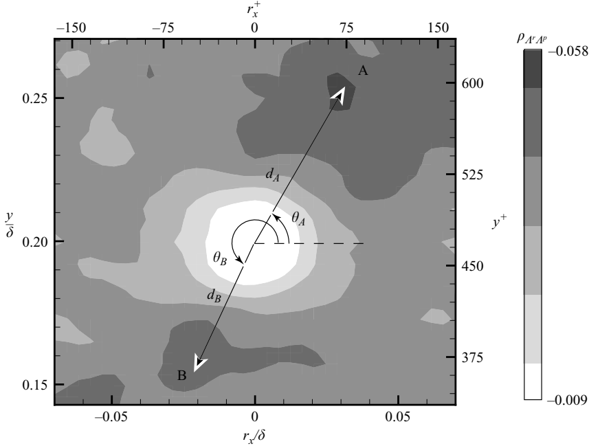
FIGURE 2. Two-point cross-correlation coefficient between \Lambda_{ci}^r and \Lambda_{ci}^p , \rho_{\Lambda^r \Lambda^p} , at y_{\text{ref}} = 0.2\delta .
