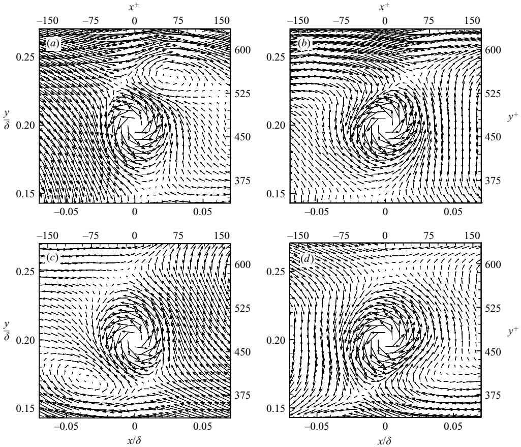
FIGURE 4. Conditionally averaged velocity fields given a retrograde vortex at y = 0.2\delta for which its closest prograde vortex is oriented in quadrants (a) one, (b) two, (c) three and (d) four relative to the retrograde core.
