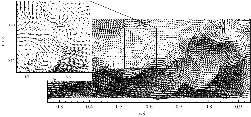
FIGURE 7. Example of a prograde hairpin vortex head (labelled A) oriented at approximately 255^\circ relative to a neighbouring retrograde vortex (labelled B), as visualized by Galilean decomposition of an instantaneous velocity realization with U_c = 0.79U_\infty .
