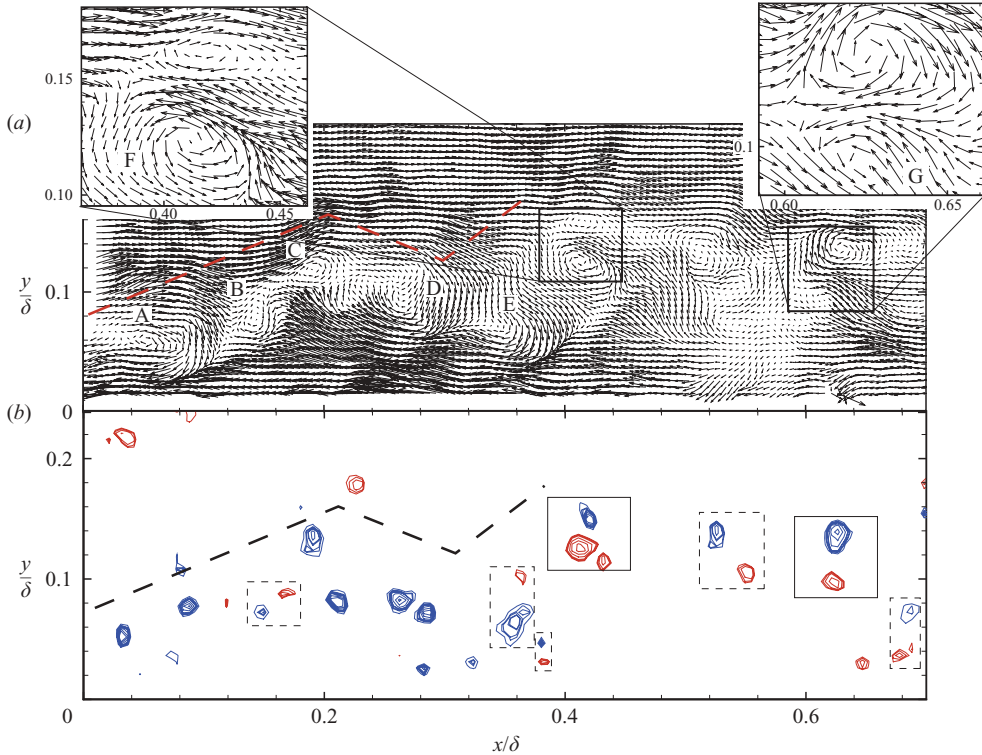
FIGURE 1. (a) Galilean-decomposed velocity field in the streamwise–wall-normal plane at Re_\tau = 2350 with U_c = 0.81U_\infty . (b) Retrograde (red) and prograde (blue) \Lambda_{ci} calculated from the velocity field in (a). The dashed line highlights the tent-like interface of the visualized packet.
