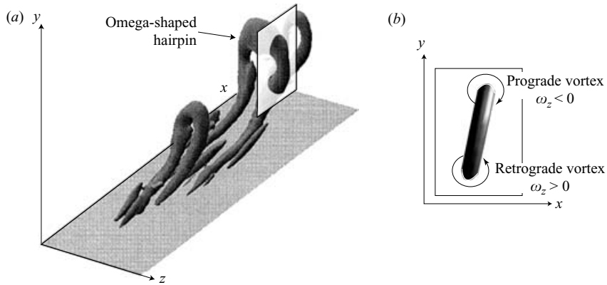
FIGURE 6. (a) Three-dimensional visualization of a hairpin vortex packet, adapted from Zhou et al. (1999), illustrating the existence of omega-shaped hairpin structures. (b) Spatial signature revealed if the structure in (a) were sliced through one of its shoulders by a streamwise–wall-normal measurement plane.
